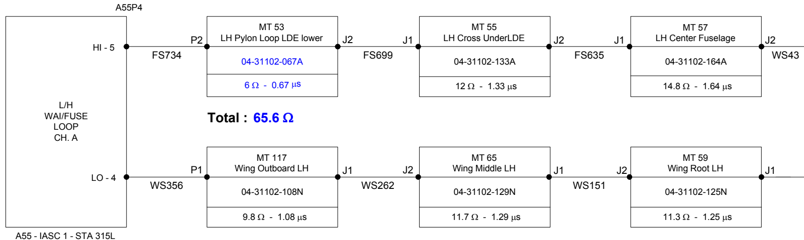
Schematics CH350
