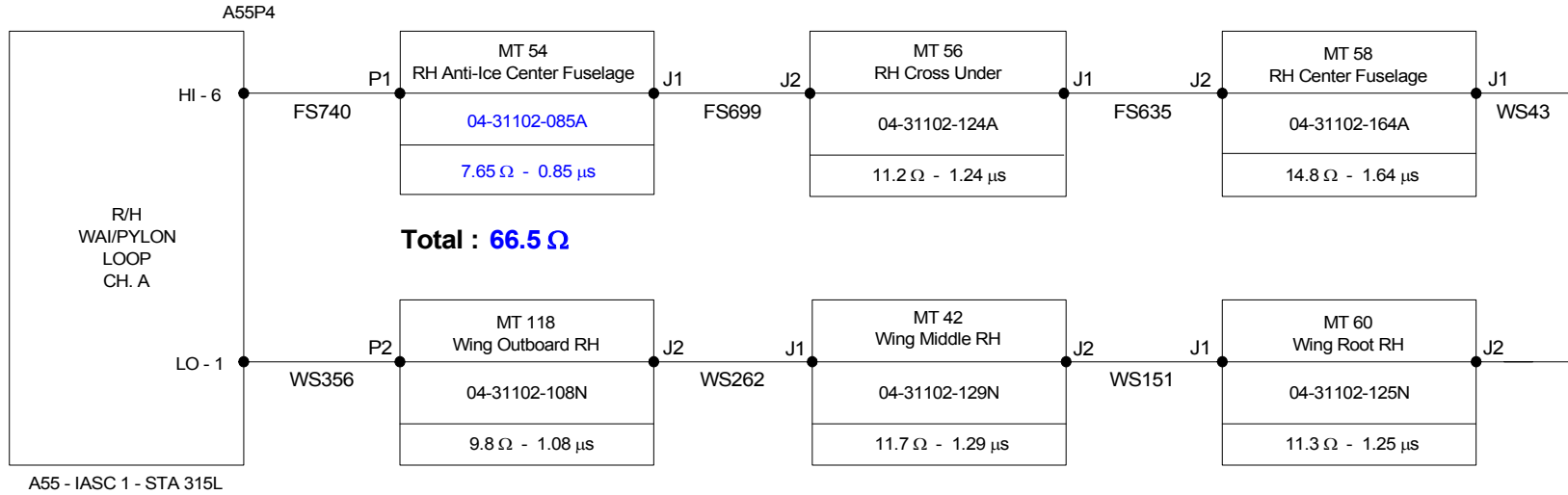
Schematics CH350
